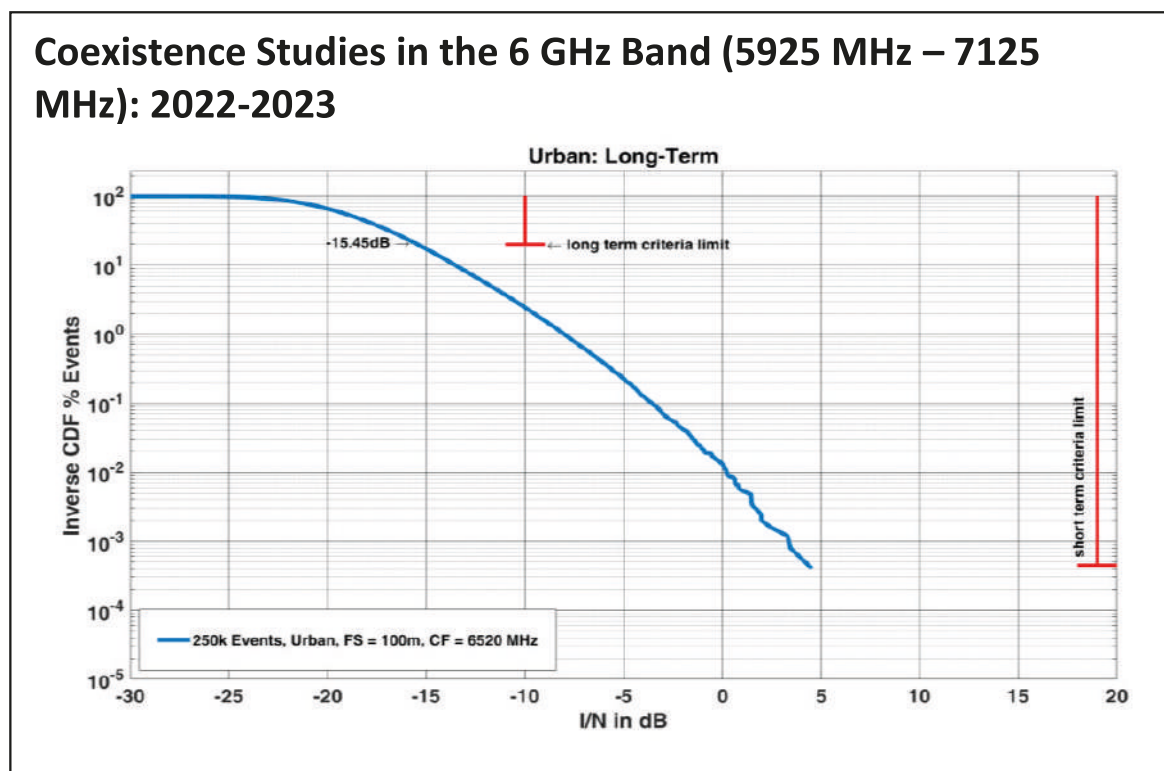
Figure 5: Long-term simulation scenario for 6 GHz Coexistence
